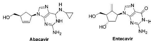
Figure 1. Examples of carbannucleosides.
