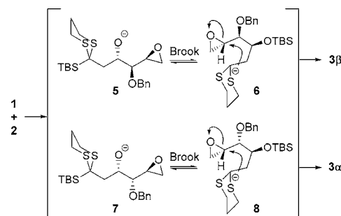
Scheme 2. Mechanism of the Carbacyclization
