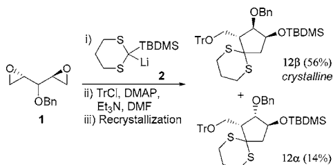
Scheme 3. Separation of the Diastereoisomers after Tritylation
