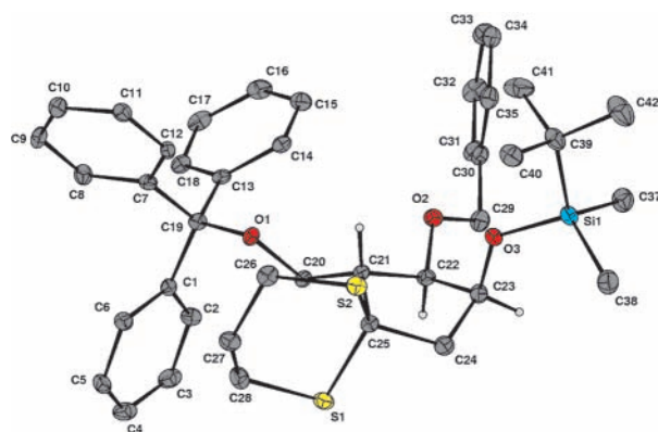
Figure 2. ORTEP representation of the crystal structure of 12β .
